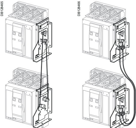
Interlocking with connecting rods
